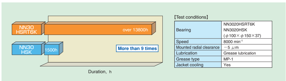
Fig. 10.7 Comparison of grease life
