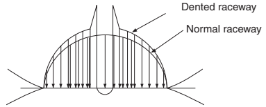
Fig. 3.4 Contact surface pressure distribution resulting from dent
